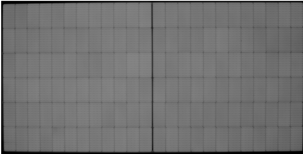
Fig. 6 EL photo of module No.2 Serial number: AS22200119604
