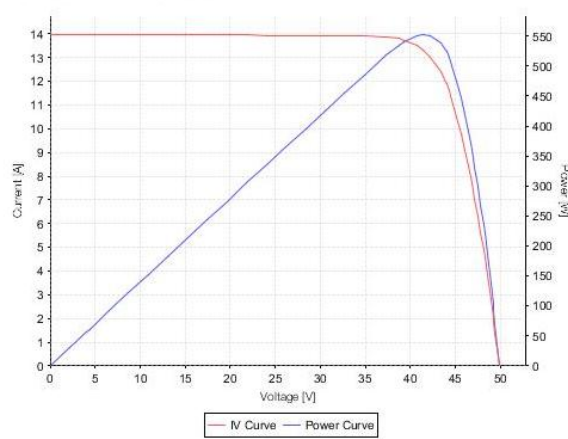
Fig. 5 IV curve of module No.1 Serial number: AS22200119604
